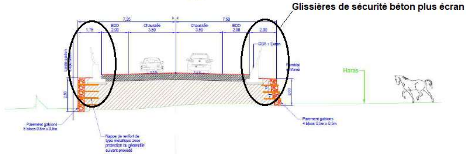
Figure 9: Coupe A8
